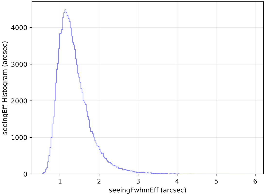
weather_cloudso31v3.4_10yrs All sky u band: seeingEff Histogram
