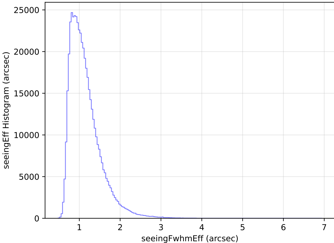
weather_cloudso31v3.4_10yrs All sky r band: seeingEff Histogram
