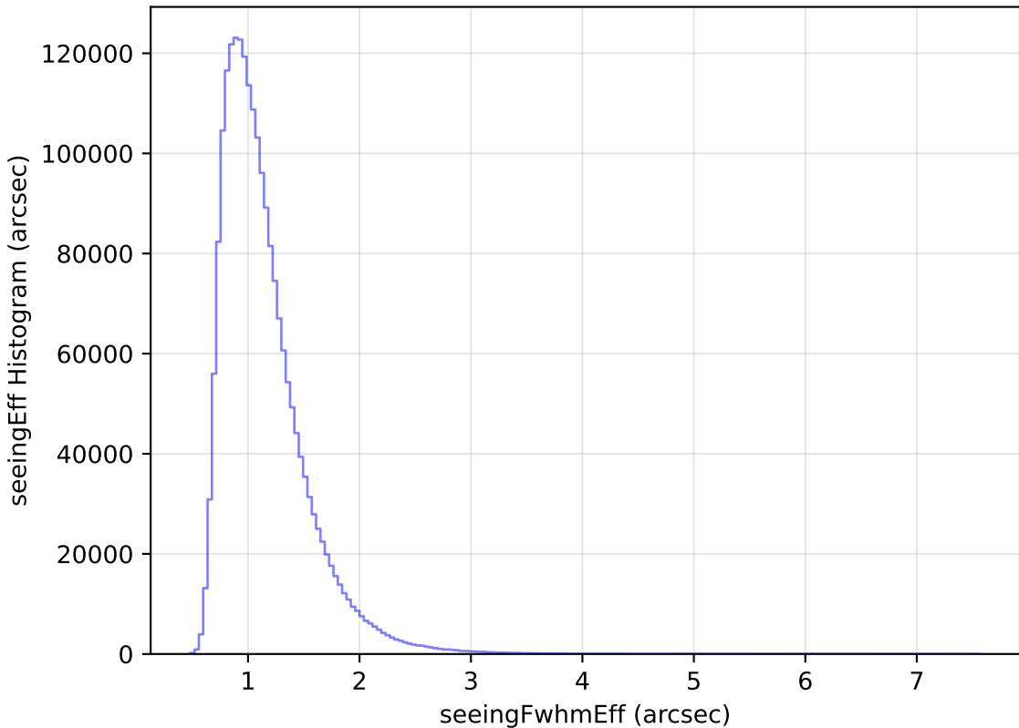
weather_cloudso31v3.4_10yrs All sky all bands: seeingEff Histogram
