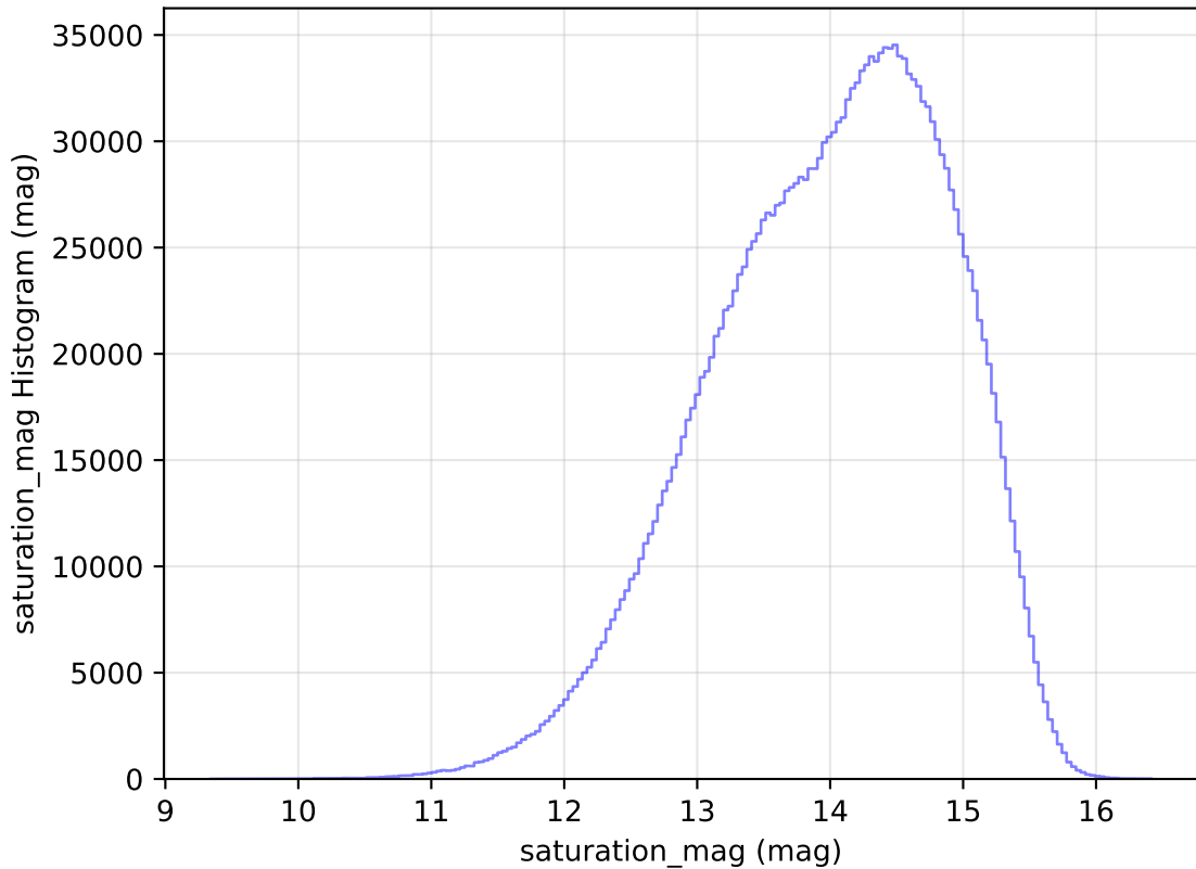
weather_cloudso31v3.4_10yrs WFD all bands: saturation_mag Histogram
