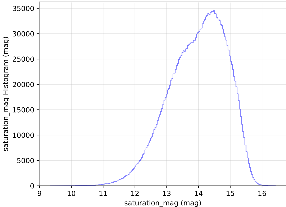
weather_cloudso31v3.4_10yrs All sky all bands: saturation_mag Histogram
