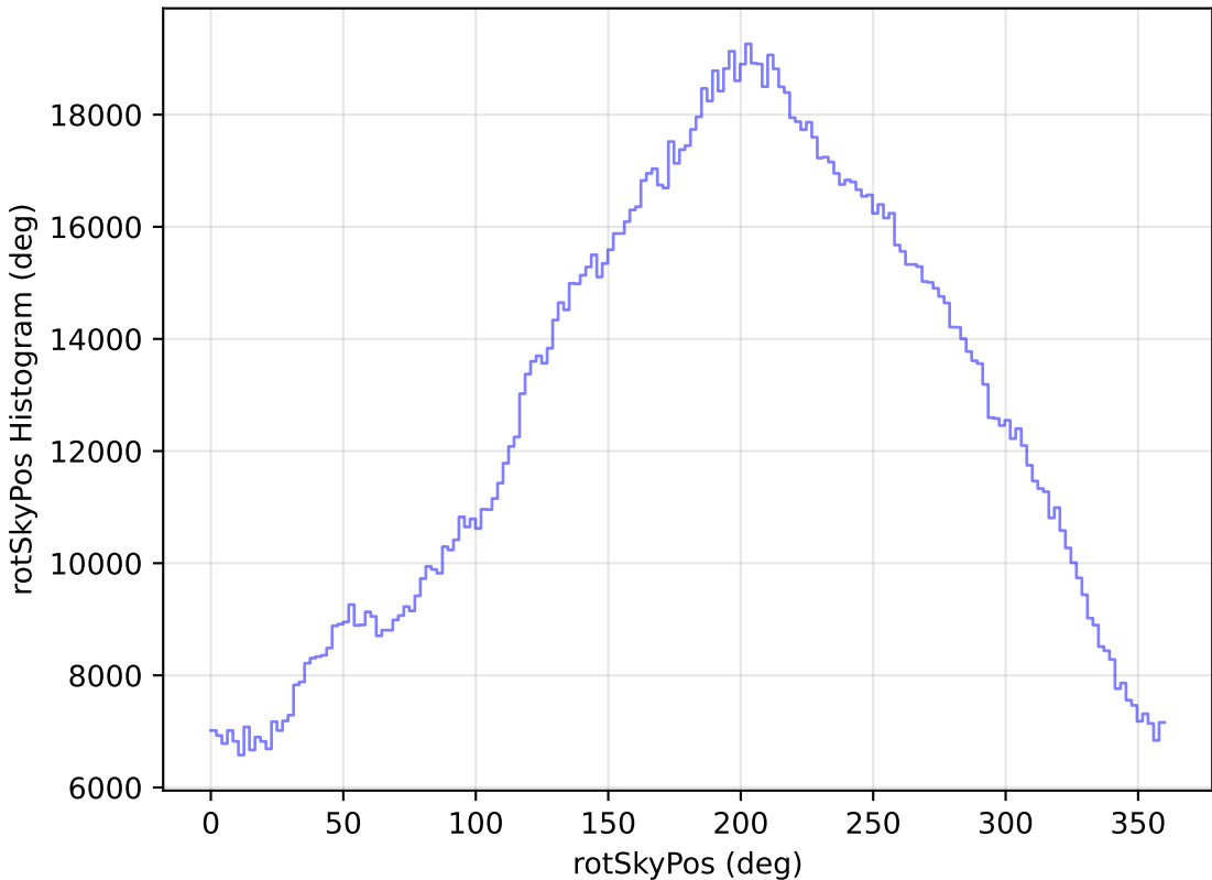
weather_cloudso31v3.4_10yrs WFD all bands: rotSkyPos Histogram
