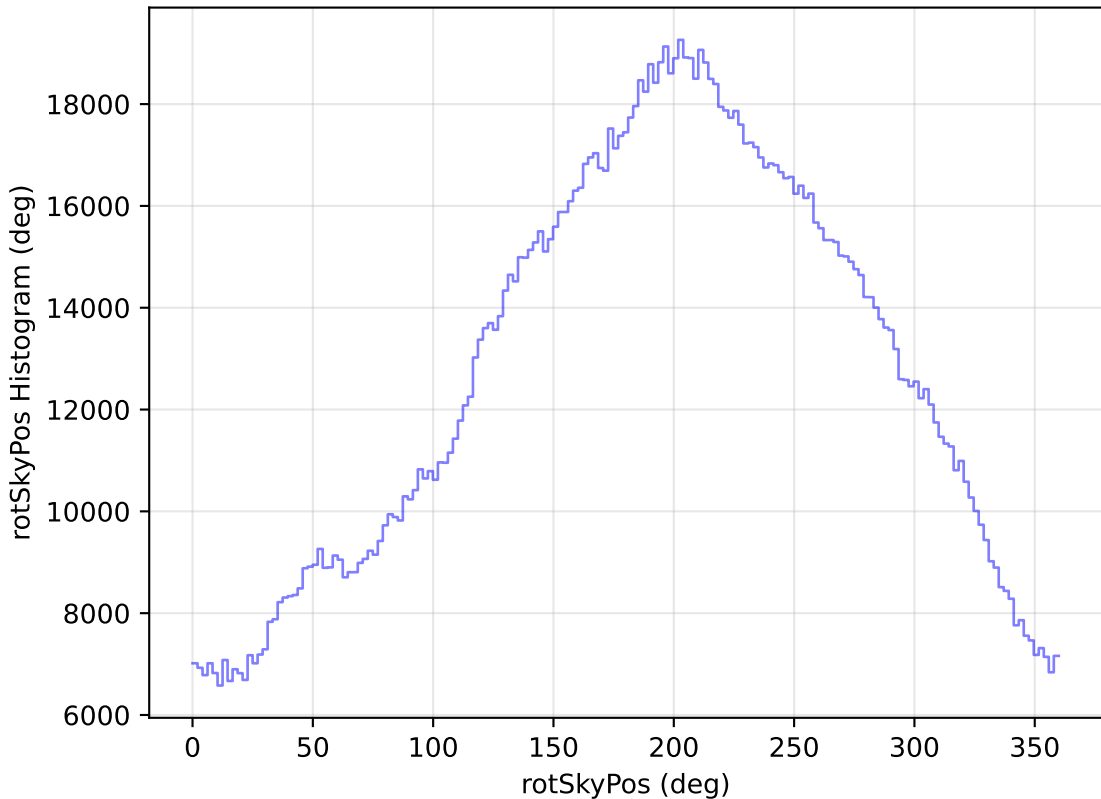
weather_cloudso31v3.4_10yrs All sky all bands: rotSkyPos Histogram
