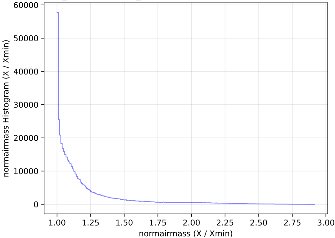
weather_cloudso31v3.4_10yrs WFD z band: normairmass Histogram
