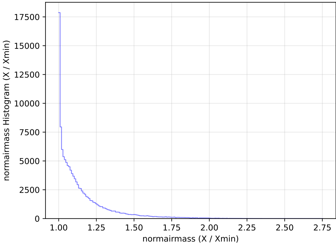
weather_cloudso31v3.4_10yrs WFD u band: normairmass Histogram
