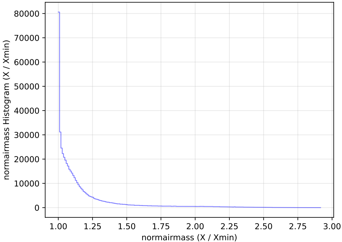
weather_cloudso31v3.4_10yrs WFD i band: normairmass Histogram
