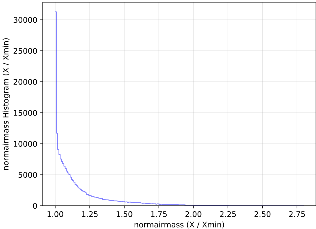
weather_cloudso31v3.4_10yrs WFD g band: normairmass Histogram
