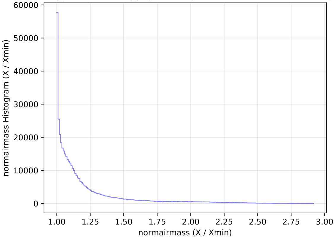
weather_cloudso31v3.4_10yrs All sky z band: normairmass Histogram
