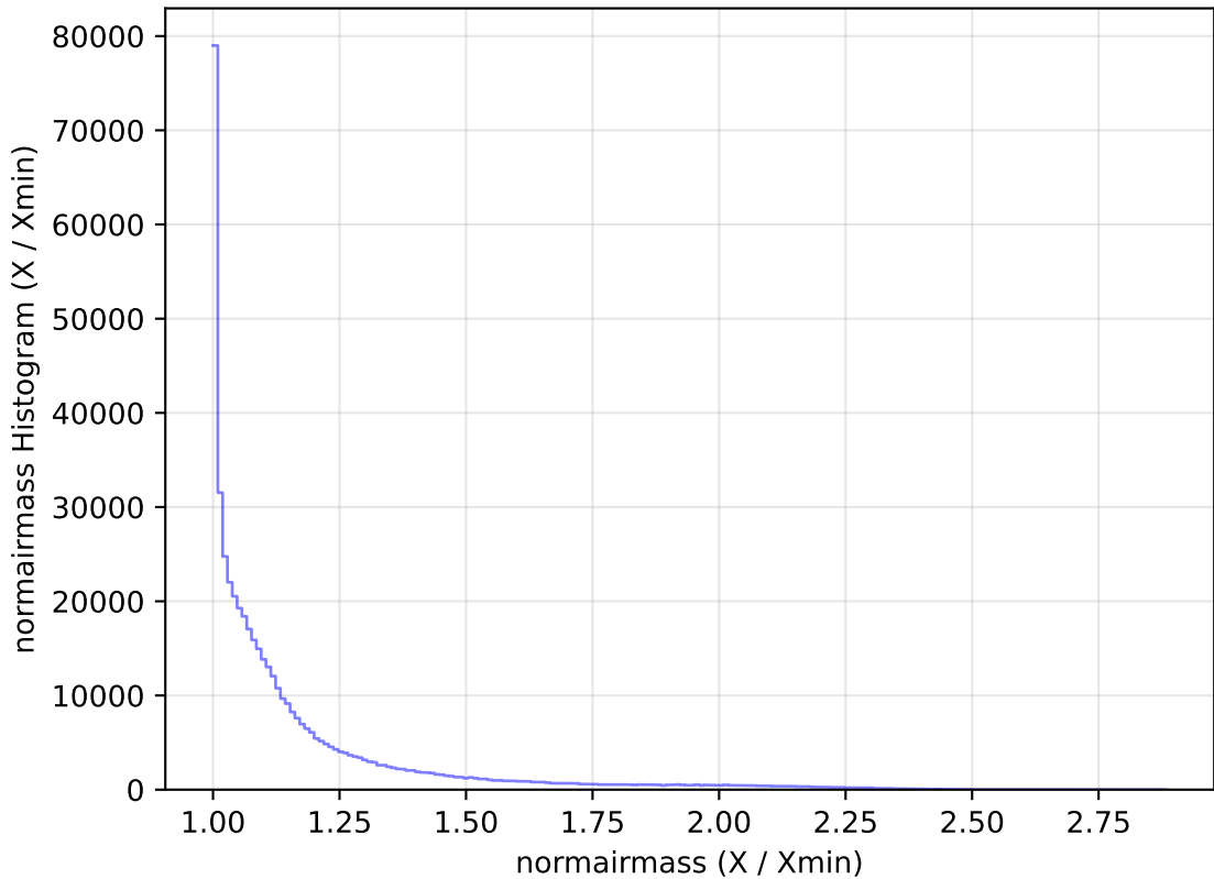
weather_cloudso31v3.4_10yrs All sky r band: normairmass Histogram
