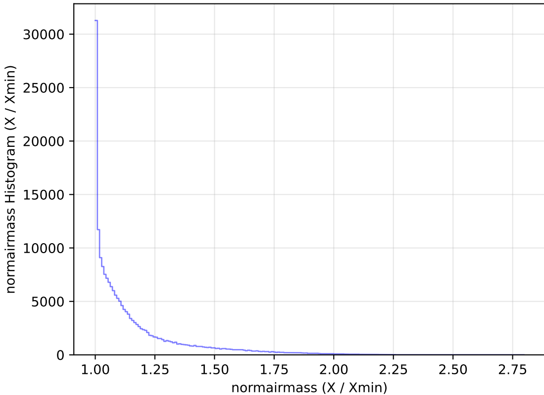
weather_cloudso31v3.4_10yrs All sky g band: normairmass Histogram
