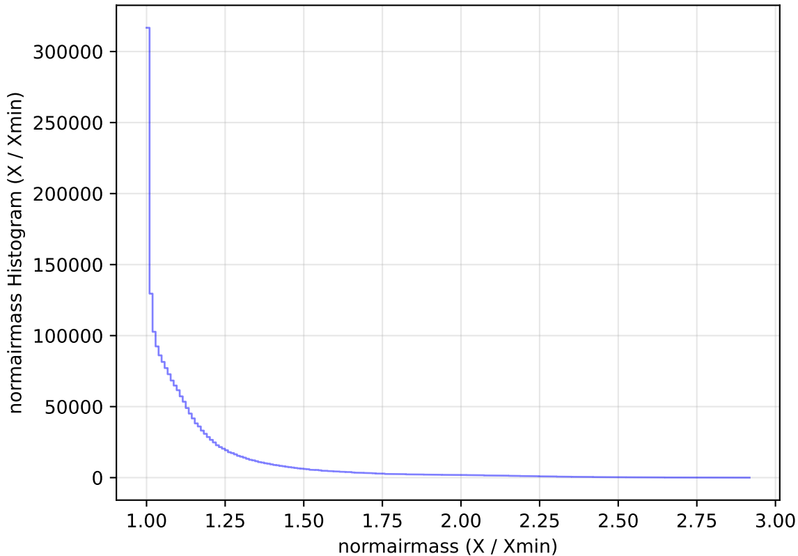
weather_cloudso31v3.4_10yrs All sky all bands: normairmass Histogram
