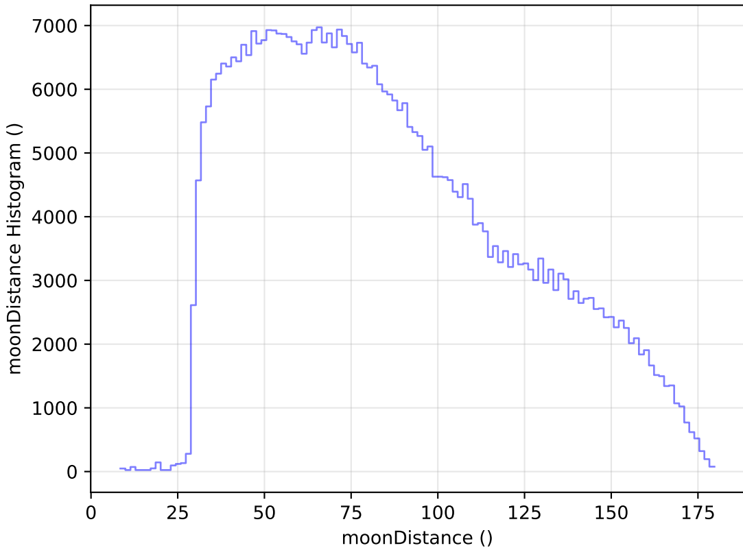
weather_cloudso31v3.4_10yrs WFD z band: moonDistance Histogram
