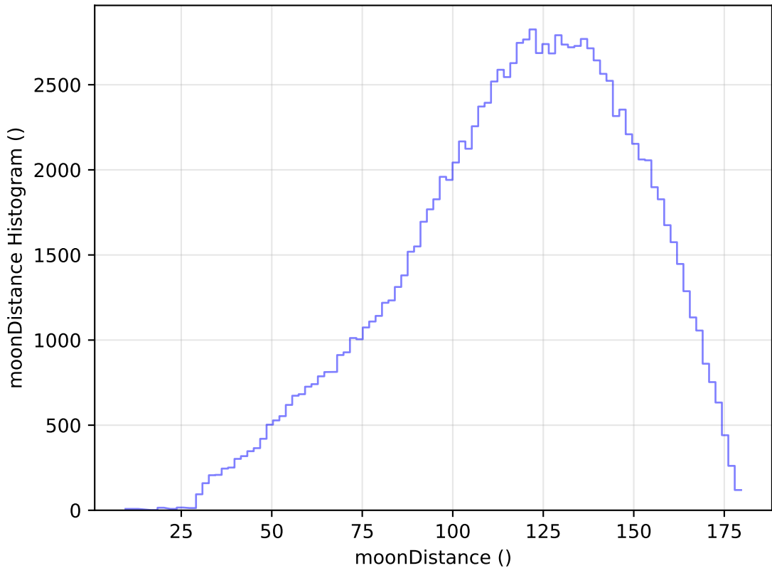
weather_cloudso31v3.4_10yrs WFD u band: moonDistance Histogram
