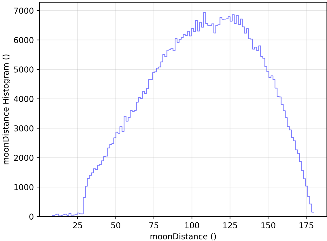
weather_cloudso31v3.4_10yrs WFD r band: moonDistance Histogram
