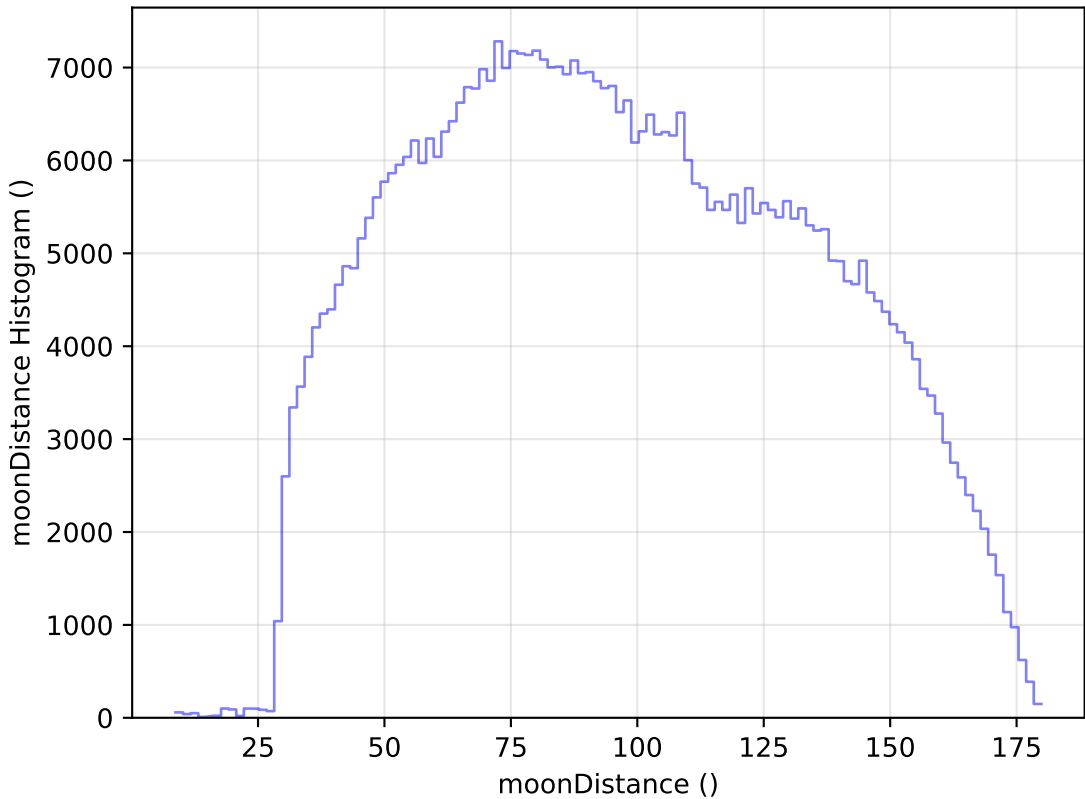
weather_cloudso31v3.4_10yrs WFD i band: moonDistance Histogram
