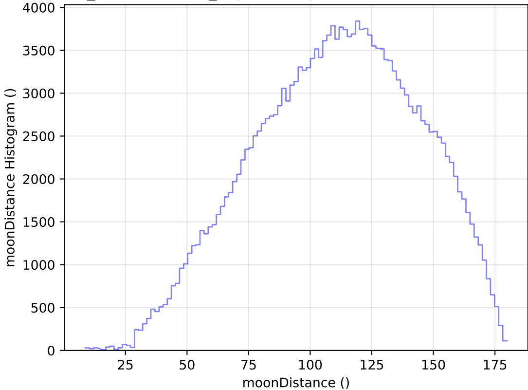
weather_cloudso31v3.4_10yrs WFD g band: moonDistance Histogram
