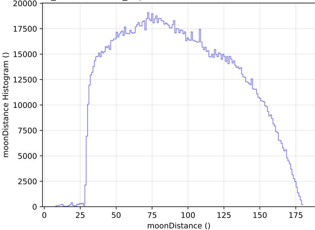
weather_cloudso31v3.4_10yrs WFD all bands: moonDistance Histogram
