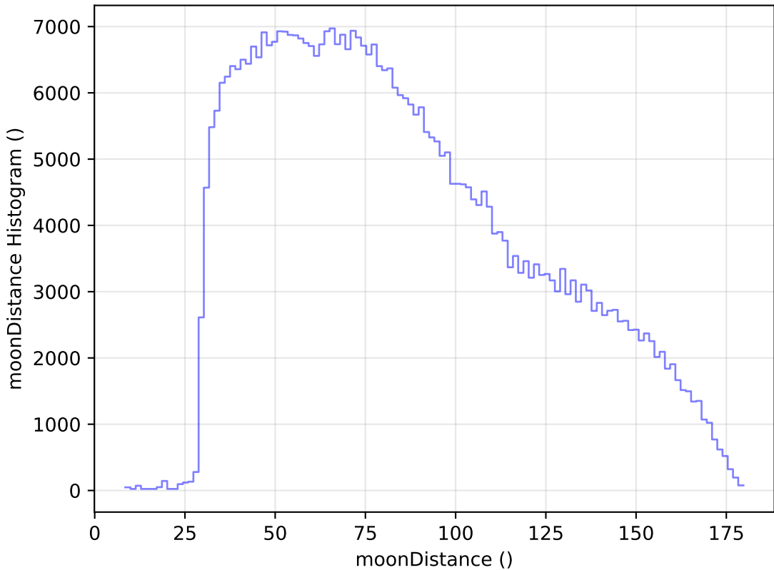
weather_cloudso31v3.4_10yrs All sky z band: moonDistance Histogram
