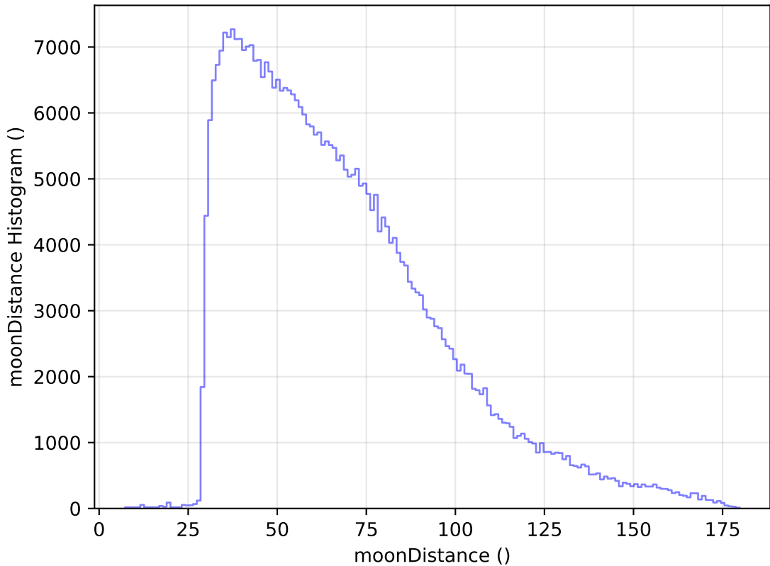
weather_cloudso31v3.4_10yrs All sky y band: moonDistance Histogram
