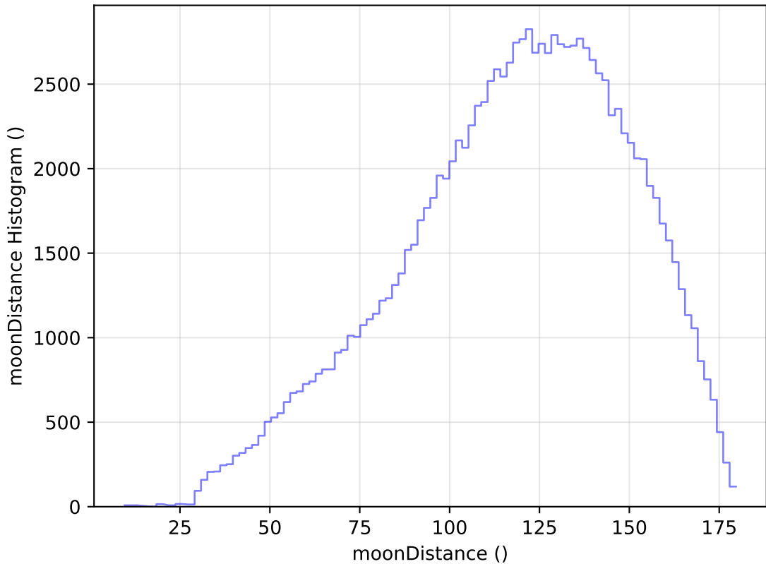
weather_cloudso31v3.4_10yrs All sky u band: moonDistance Histogram
