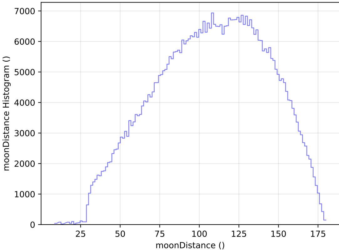
weather_cloudso31v3.4_10yrs All sky r band: moonDistance Histogram
