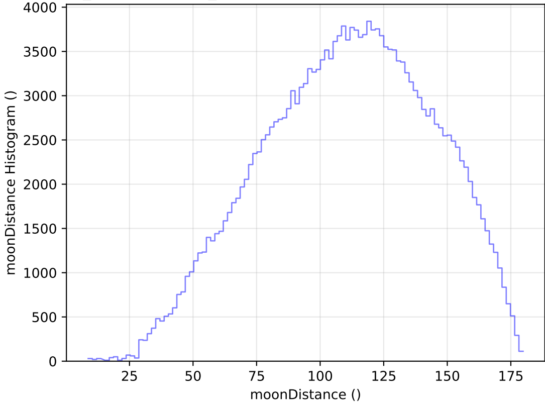
weather_cloudso31v3.4_10yrs All sky g band: moonDistance Histogram
