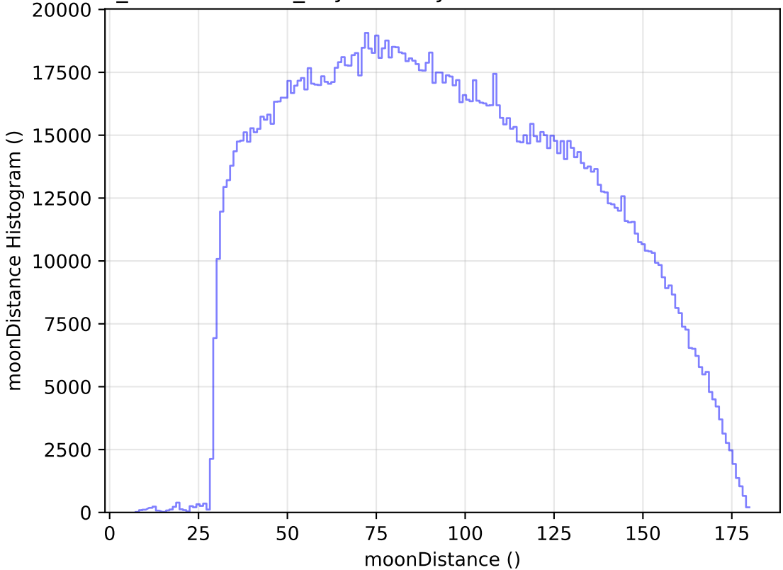
weather_cloudso31v3.4_10yrs All sky all bands: moonDistance Histogram
