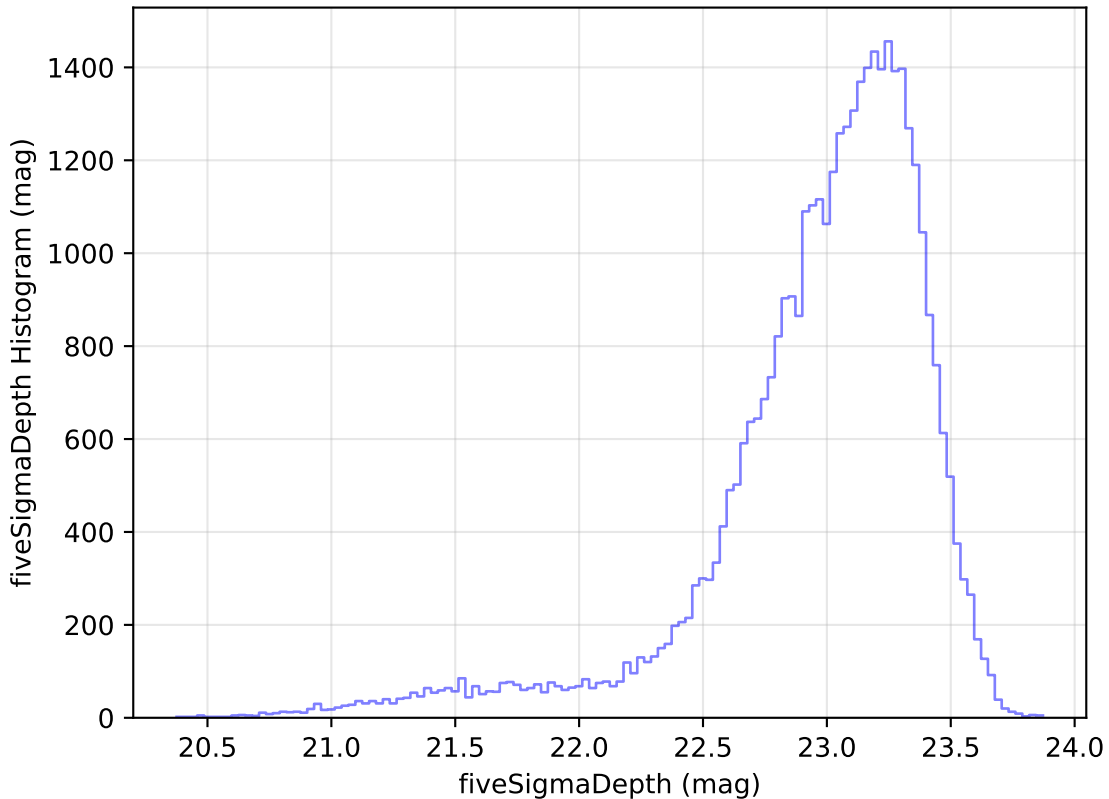
weather_cloudso31v3.4_10yrs Yr 1 z band: fiveSigmaDepth Histogram
