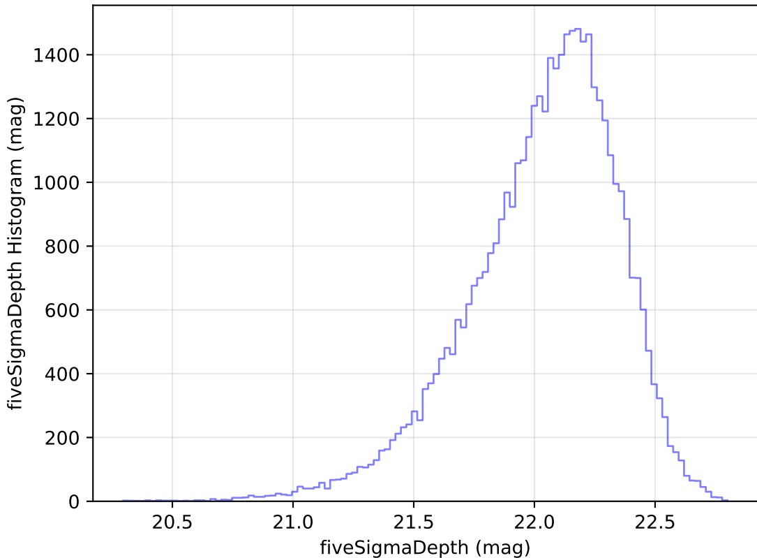
weather_cloudso31v3.4_10yrs Yr 1 y band: fiveSigmaDepth Histogram
