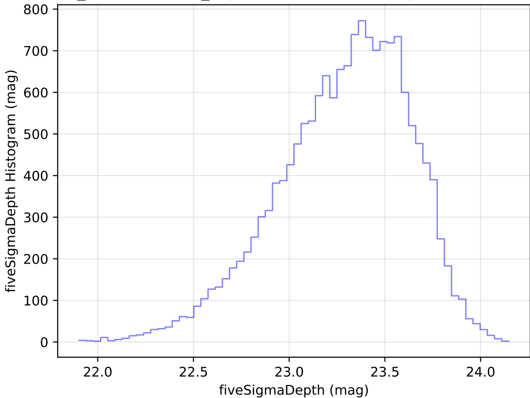
weather_cloudso31v3.4_10yrs Yr 1 u band: fiveSigmaDepth Histogram
