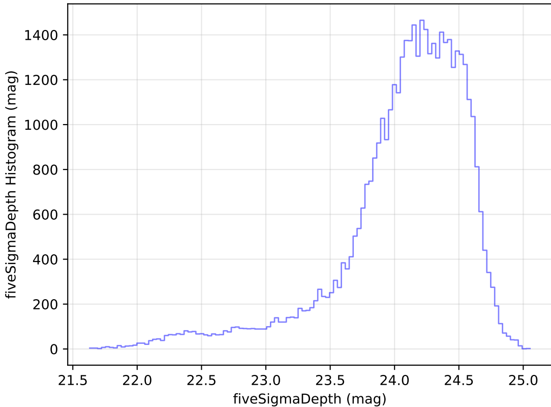
weather_cloudso31v3.4_10yrs Yr 1 r band: fiveSigmaDepth Histogram
