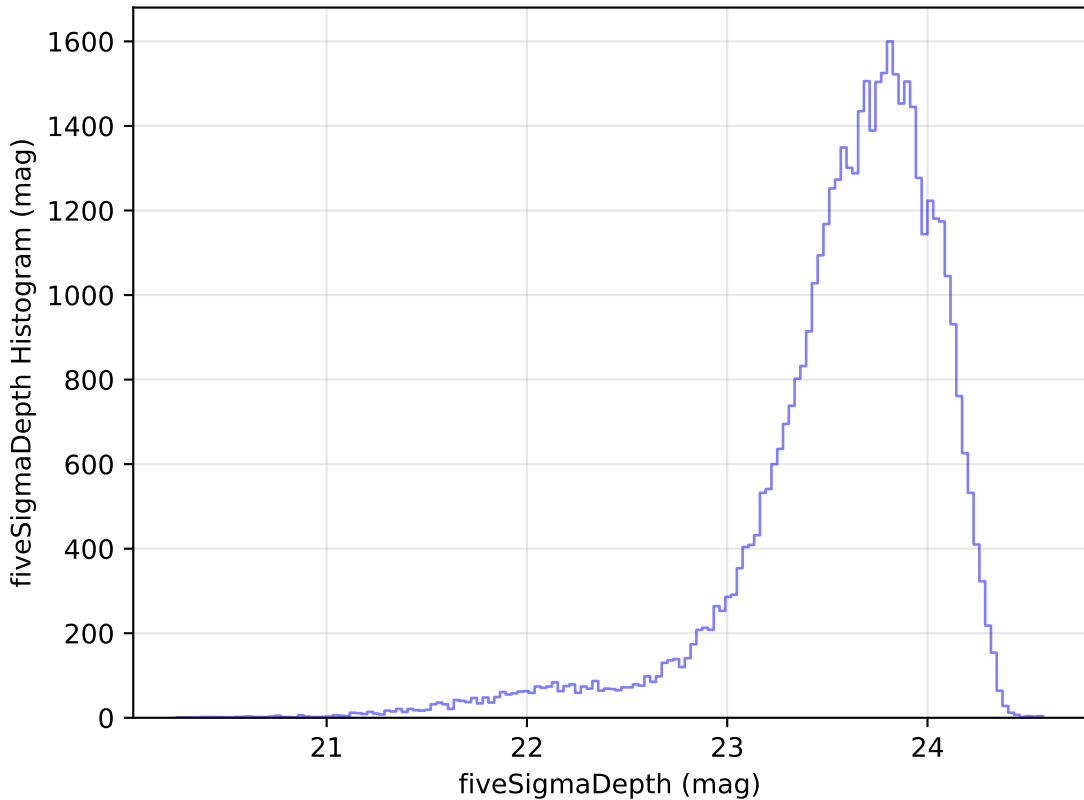
weather_cloudso31v3.4_10yrs Yr 1 i band: fiveSigmaDepth Histogram
