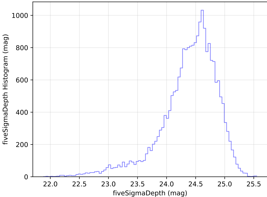
weather_cloudso31v3.4_10yrs Yr 1 g band: fiveSigmaDepth Histogram
