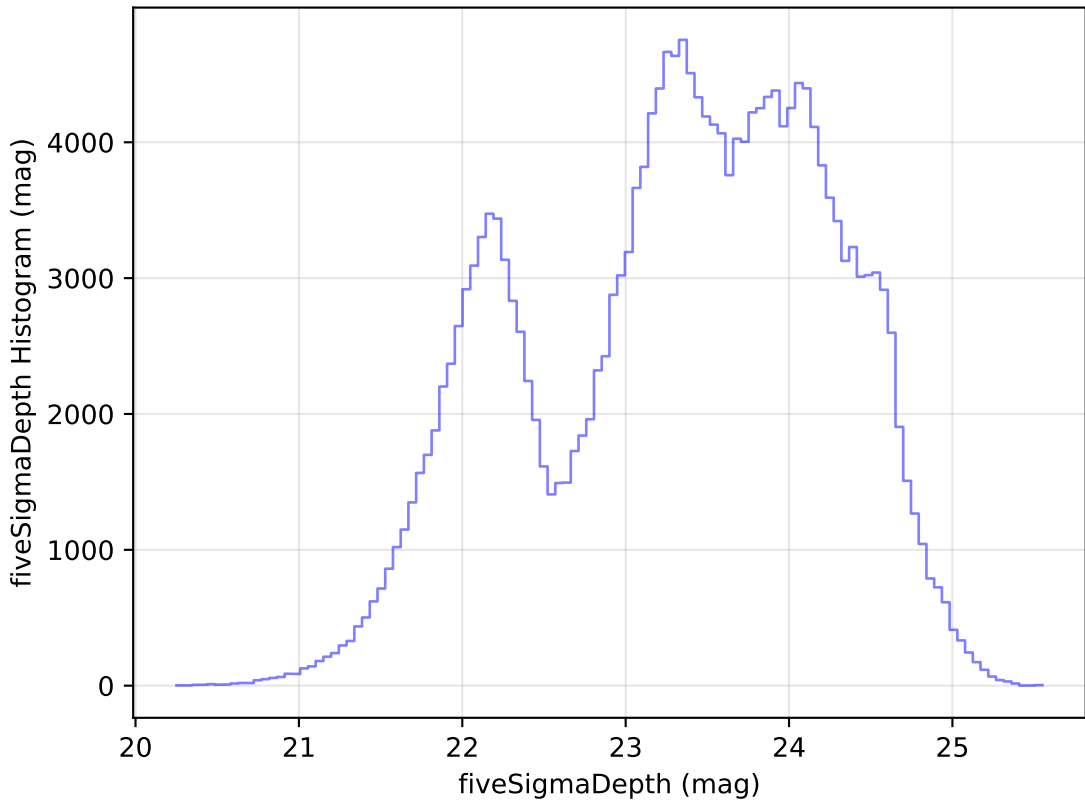
weather_cloudso31v3.4_10yrs Yr 1 all bands: fiveSigmaDepth Histogram
