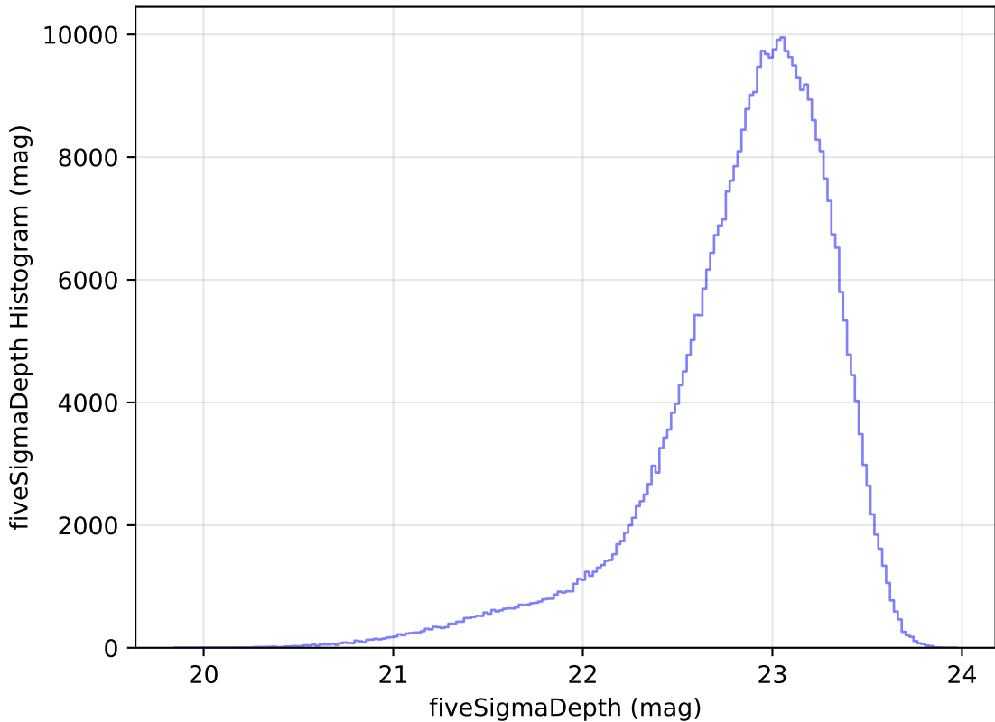
weather_cloudso31v3.4_10yrs WFD z band: fiveSigmaDepth Histogram
