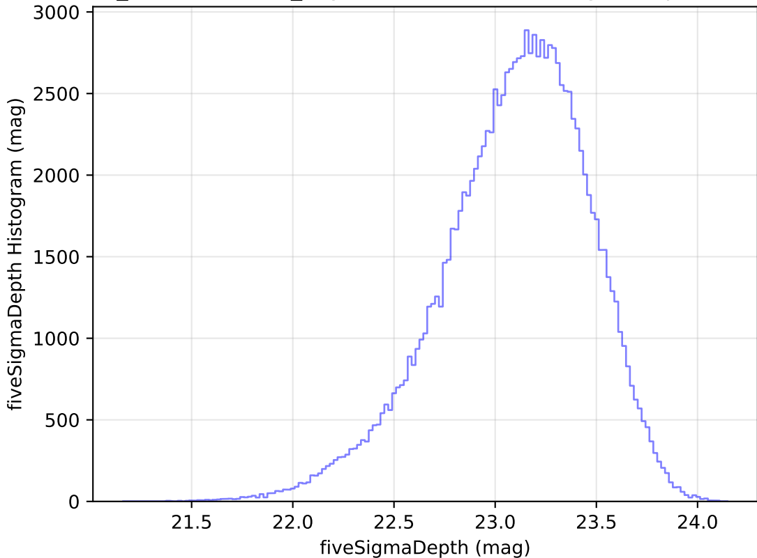
weather_cloudso31v3.4_10yrs WFD u band: fiveSigmaDepth Histogram
