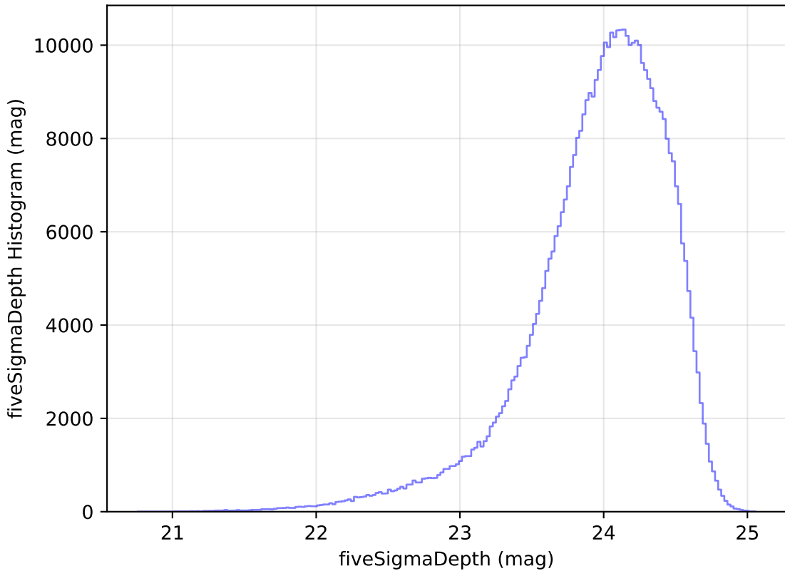
weather_cloudso31v3.4_10yrs WFD r band: fiveSigmaDepth Histogram
