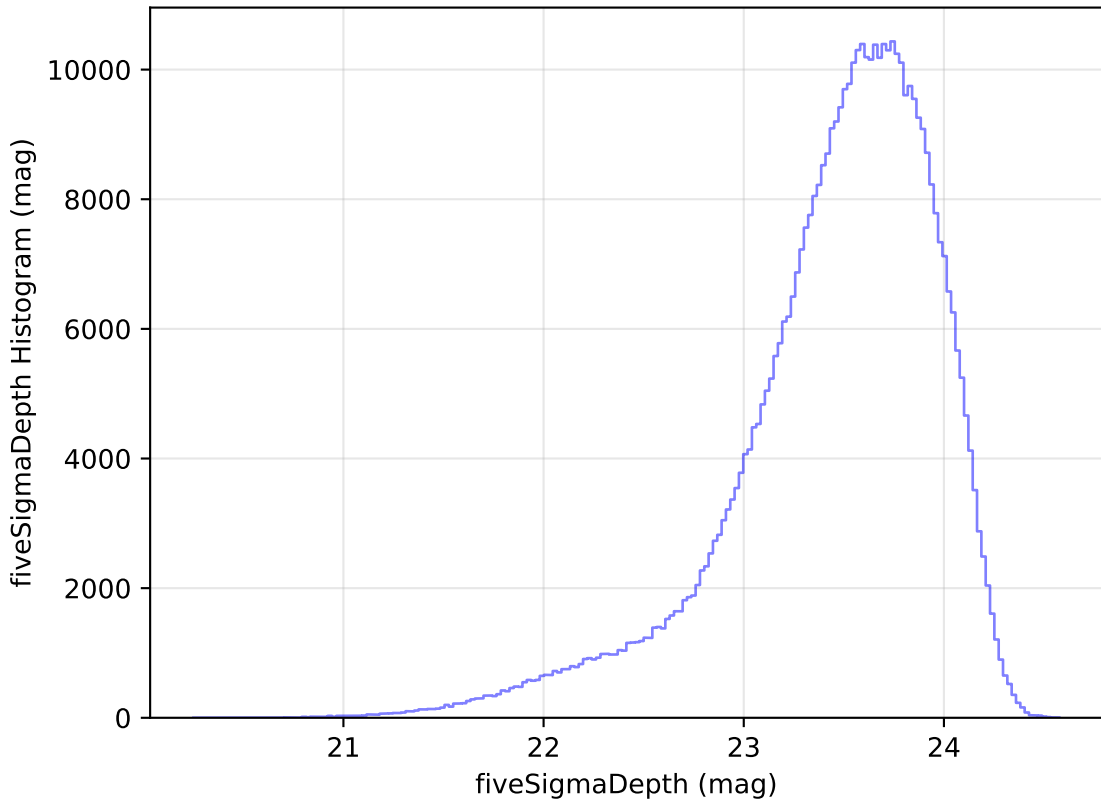
weather_cloudso31v3.4_10yrs WFD i band: fiveSigmaDepth Histogram
