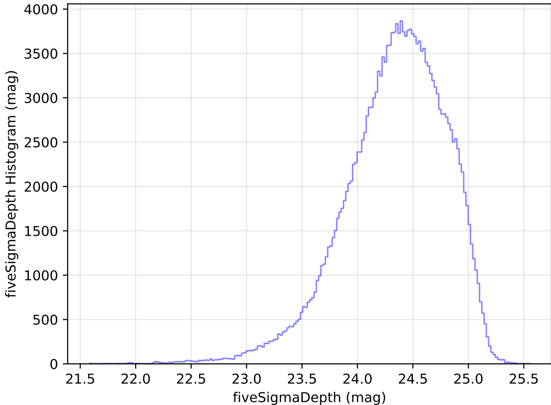
weather_cloudso31v3.4_10yrs WFD g band: fiveSigmaDepth Histogram
