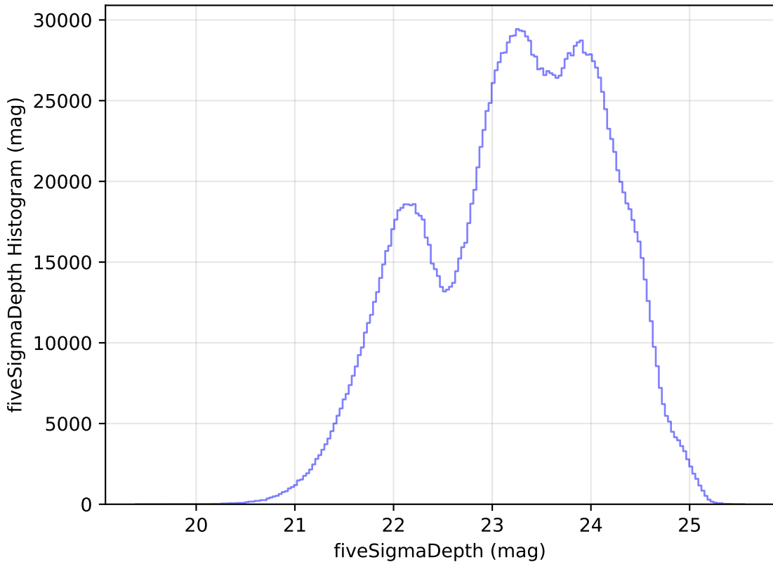
weather_cloudso31v3.4_10yrs WFD all bands: fiveSigmaDepth Histogram
