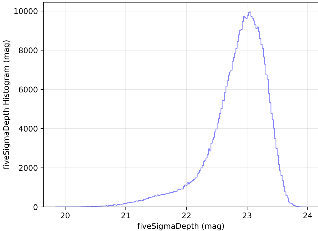
weather_cloudso31v3.4_10yrs All sky z band: fiveSigmaDepth Histogram
