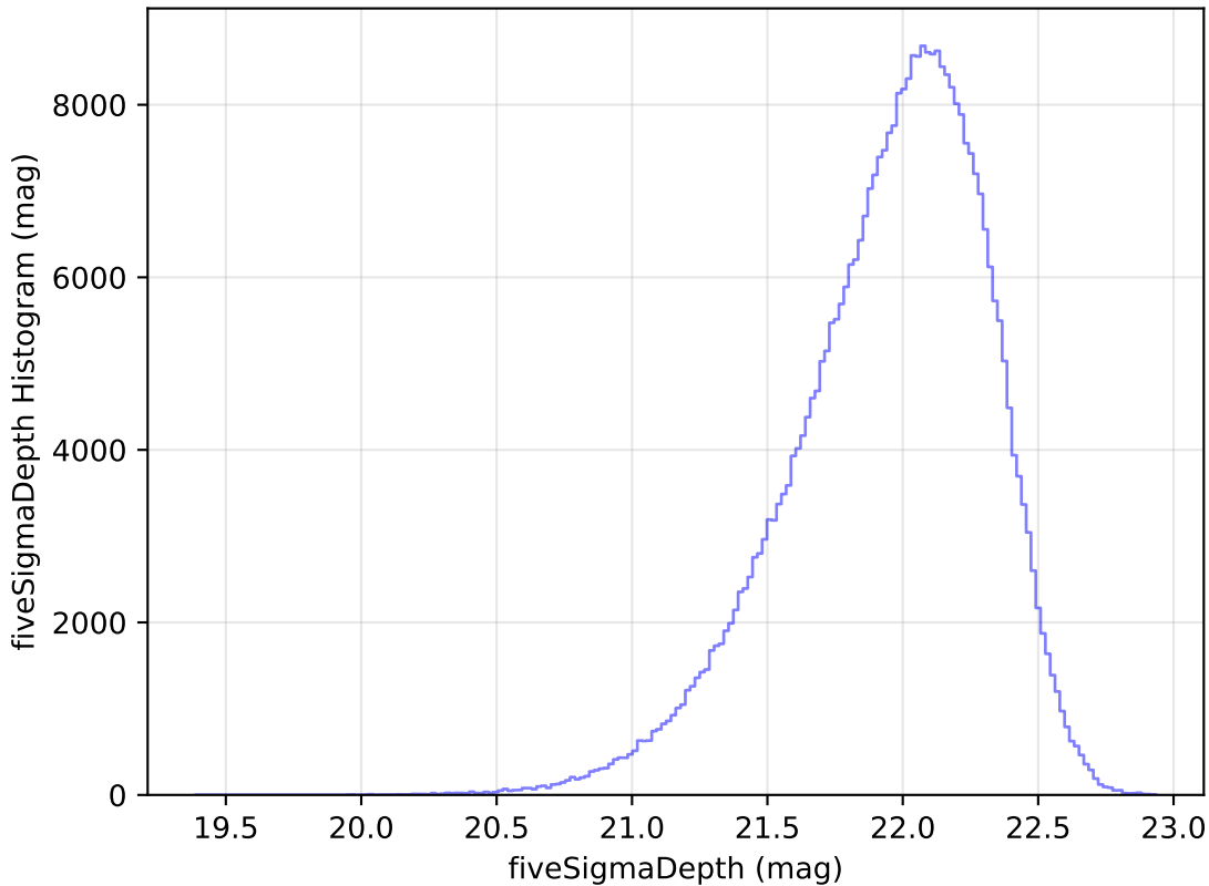
weather_cloudso31v3.4_10yrs All sky y band: fiveSigmaDepth Histogram
