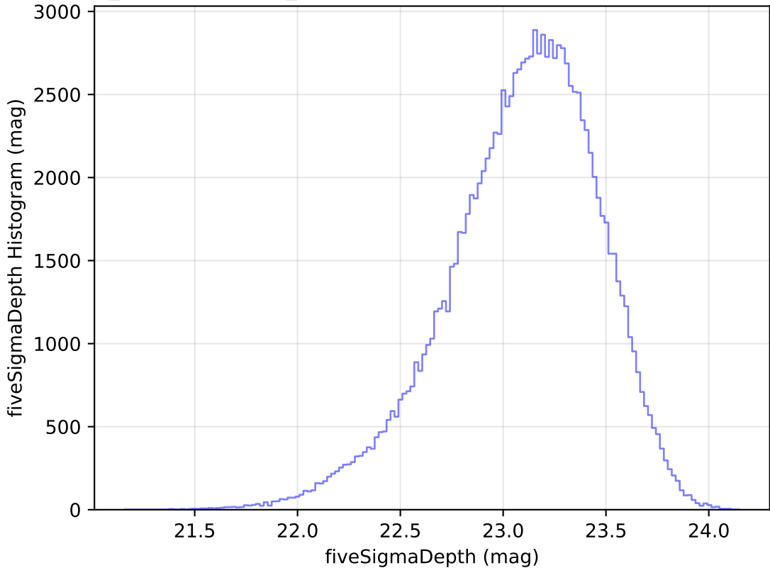
weather_cloudso31v3.4_10yrs All sky u band: fiveSigmaDepth Histogram
