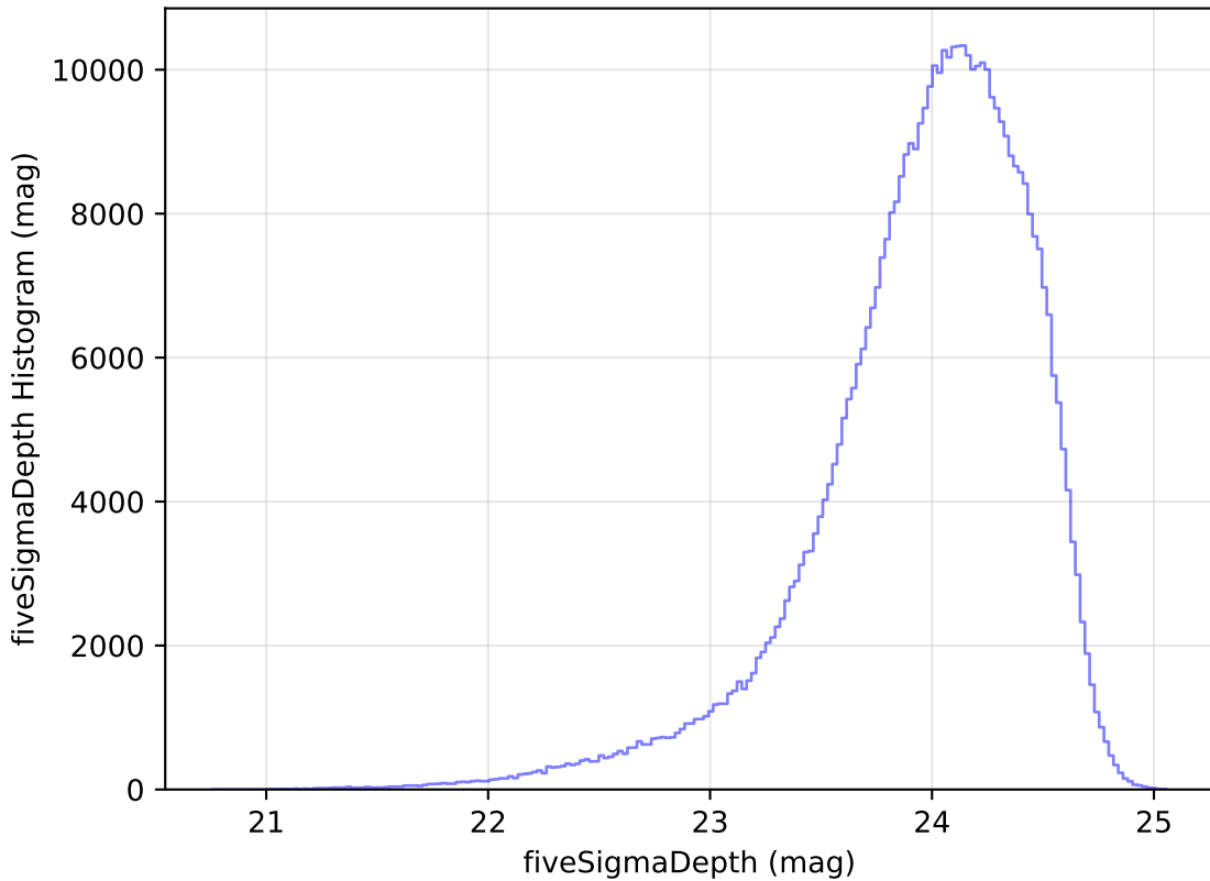
weather_cloudso31v3.4_10yrs All sky r band: fiveSigmaDepth Histogram
