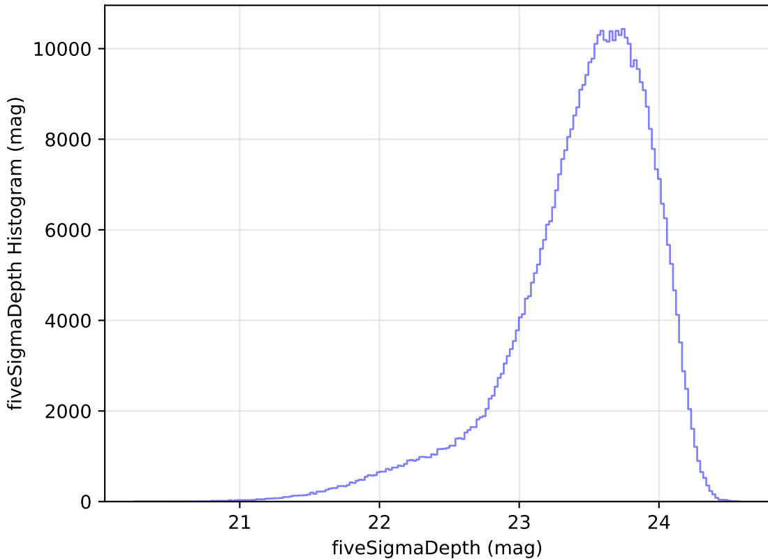
weather_cloudso31v3.4_10yrs All sky i band: fiveSigmaDepth Histogram
