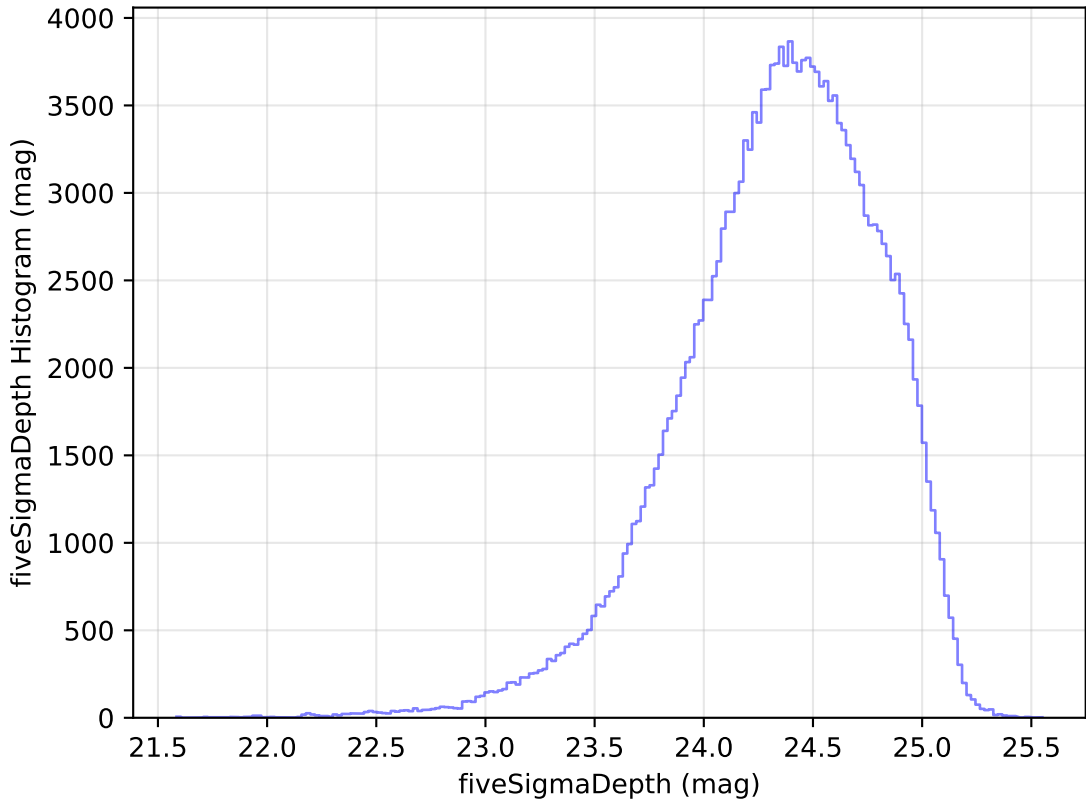
weather_cloudso31v3.4_10yrs All sky g band: fiveSigmaDepth Histogram
