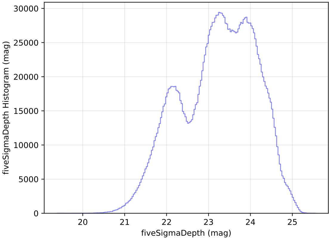
weather_cloudso31v3.4_10yrs All sky all bands: fiveSigmaDepth Histogram
