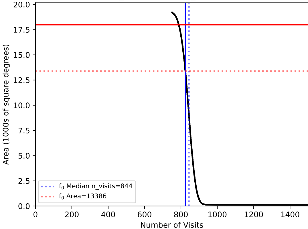
weather_cloudso31v3.4_10yrs WFD: f0
