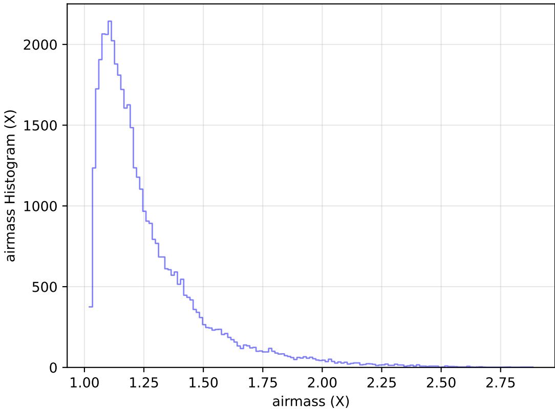
weather_cloudso31v3.4_10yrs Yr 1 y band: airmass Histogram
