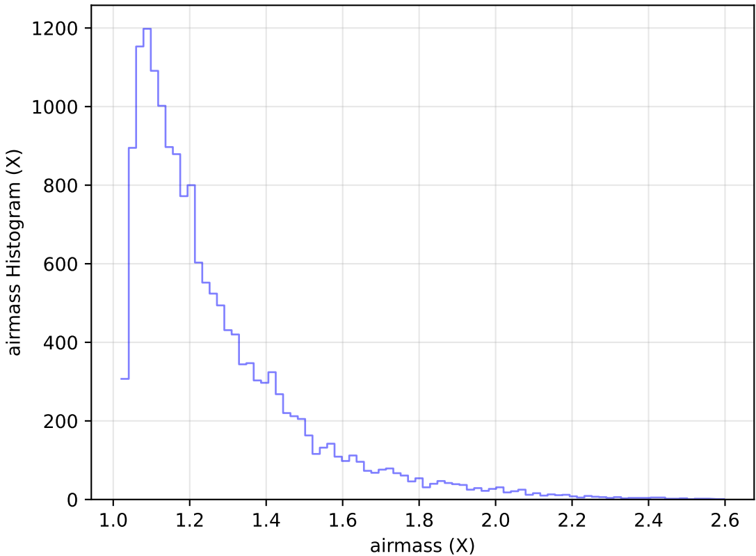
weather_cloudso31v3.4_10yrs Yr 1 u band: airmass Histogram
